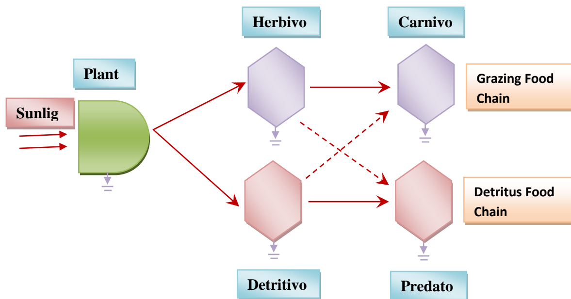
Figure 3: Y-Shaped energy flow model showing linkage between grazing and detritus food chain.
