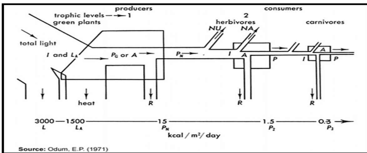
Figure 2. Linear energy flow model in an Ecosystem. (I-Total energy input, A- total assimilation, LA- Light absorbrd by plants, PG- Gross primary Productivity, PN- Net primary productivity, P-Secondary productivity, NU- Energy not used, NA- Energy not assimilated by consumer, R- respiration).
